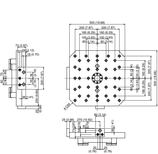
Pallet Top View Unit : mm (in.)
