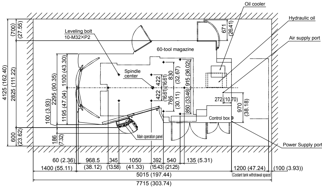
Floor Plan Unit : mm (in.)
