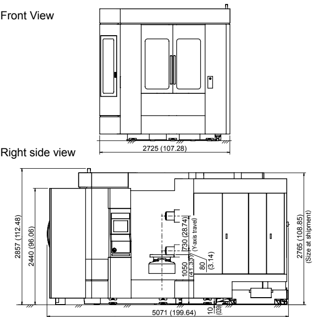
External View Unit : mm (in.)
