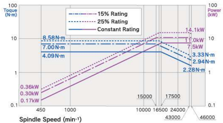
■ Spindle Motor Torque & Power Diagram
