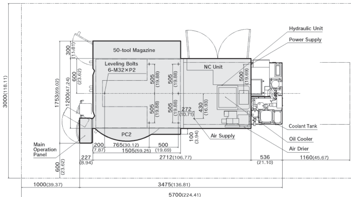
Floor Plan (50-tool Magazine with PC2) Option Units: mm (in.)
